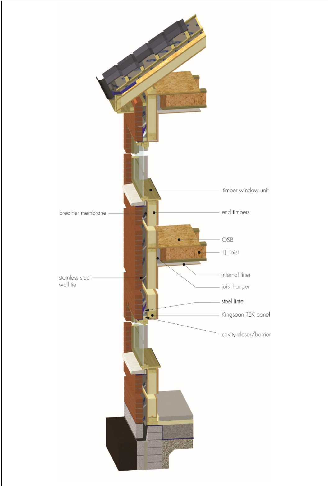
Figure 1 Typical wall and roof construction
