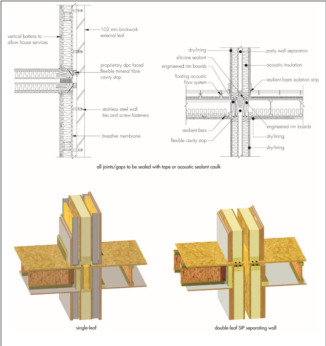
Figure 6 Separating wall details
