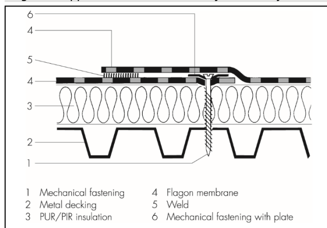
Figure 1 Application to steel decks – fastener in joint
