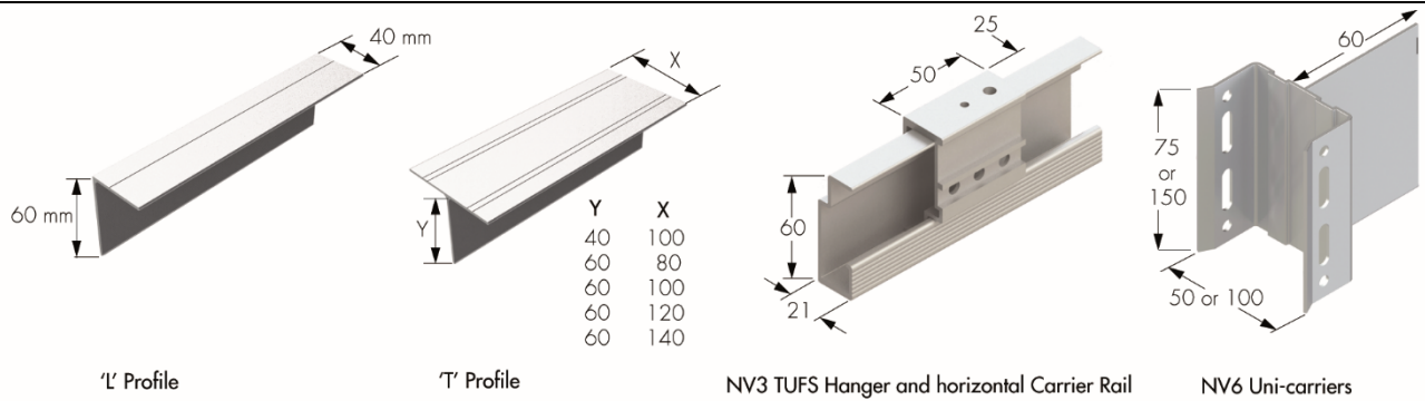
Figure 2 Component details
