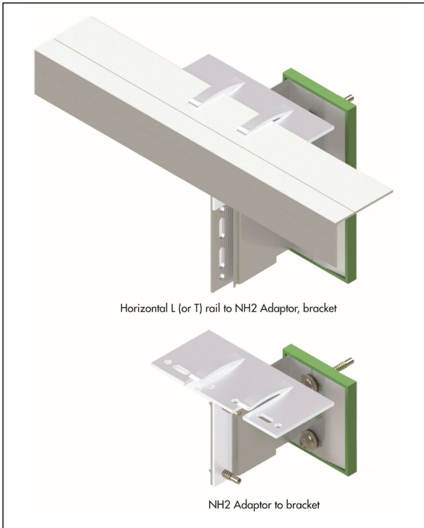
Figure 3 NH2 Adaptor
